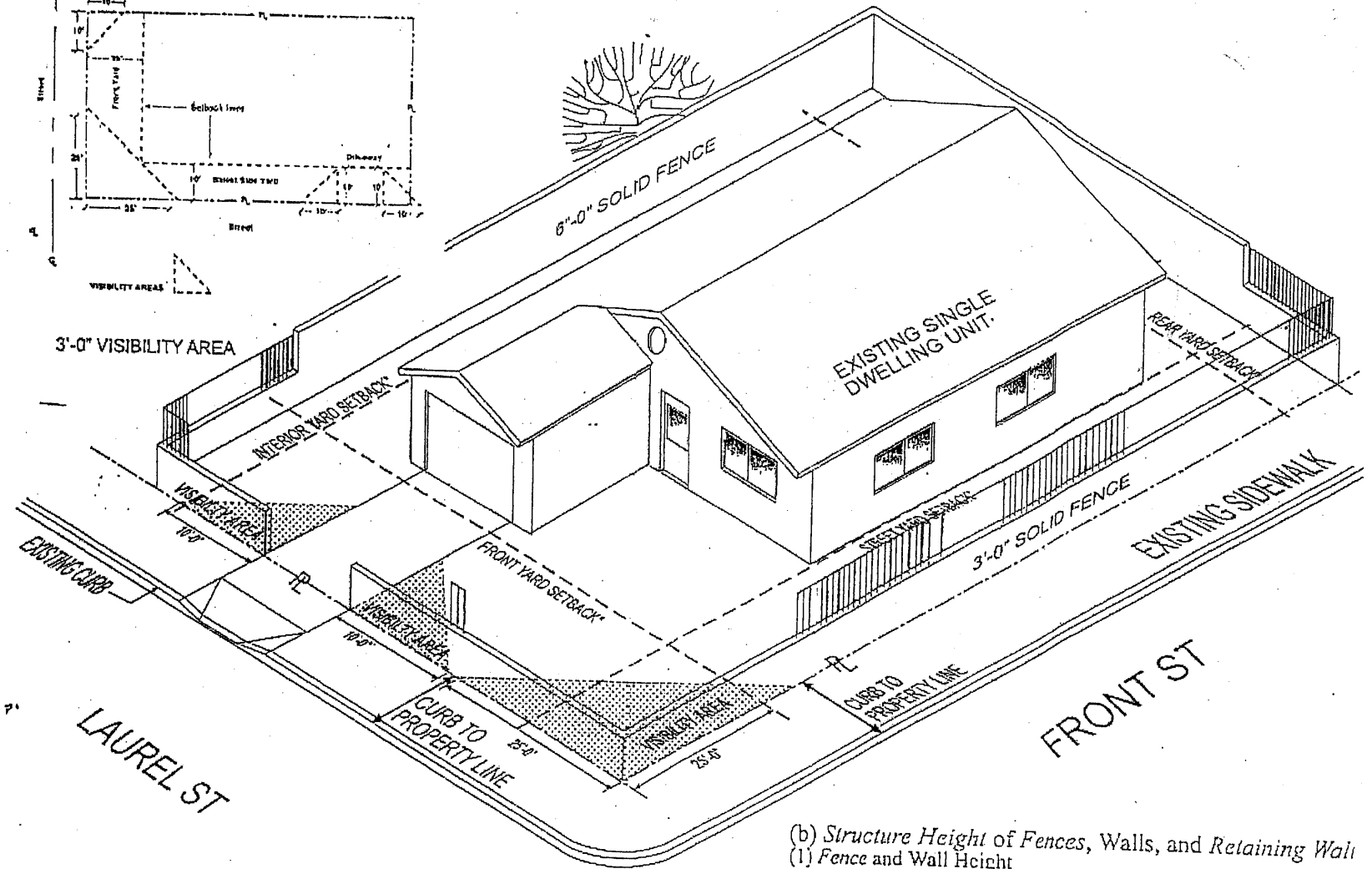
Diagram 113-02Q2 Visibility Area
